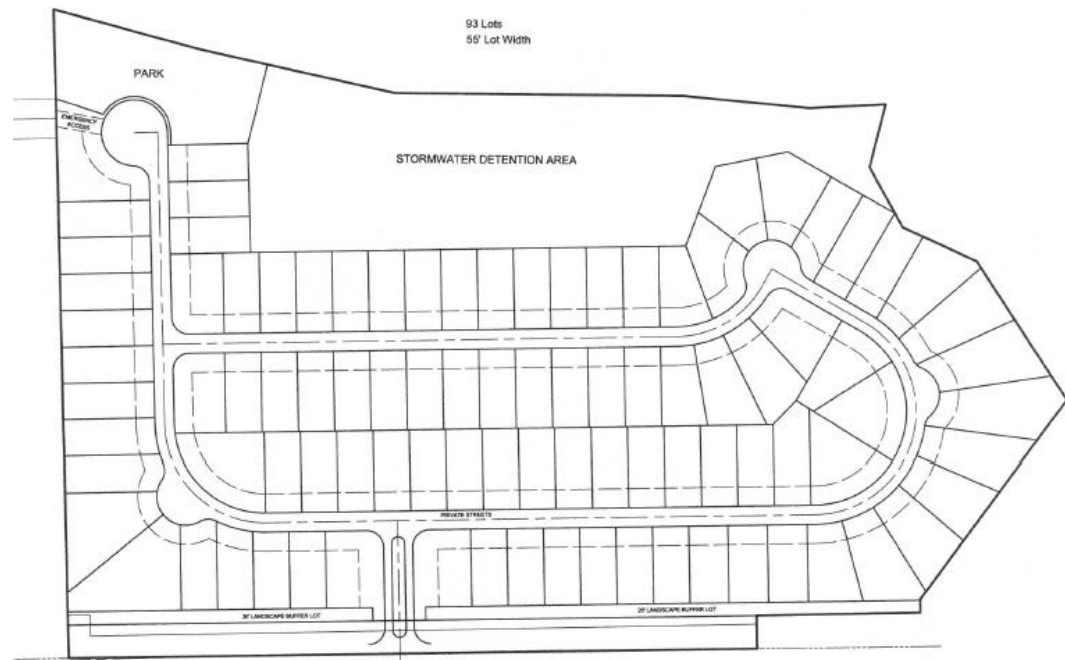
Single Family Concept Plan
